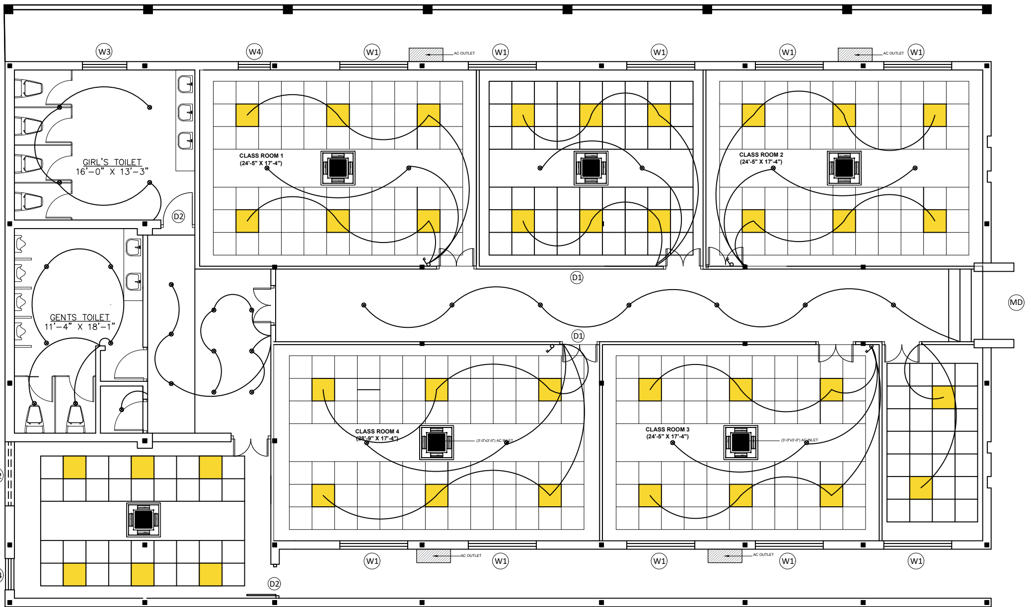
GROUND FLOOR ELECTRICAL DRAWING
